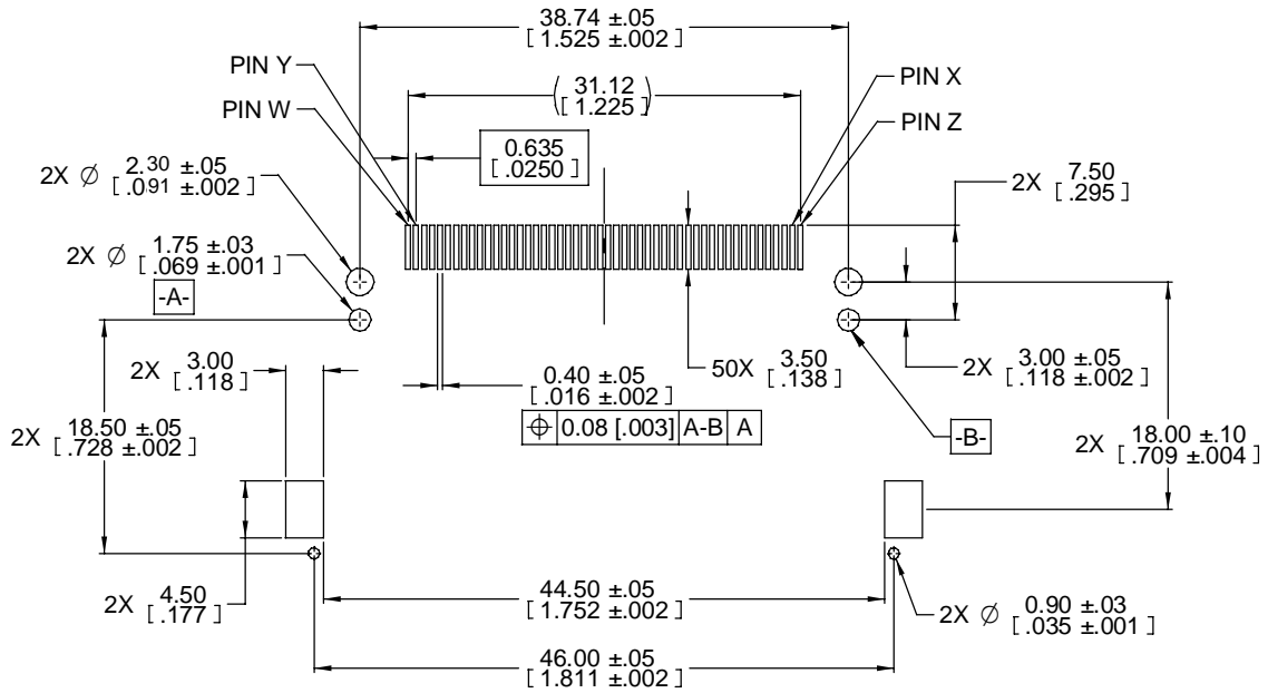
PCB LAYOUT
