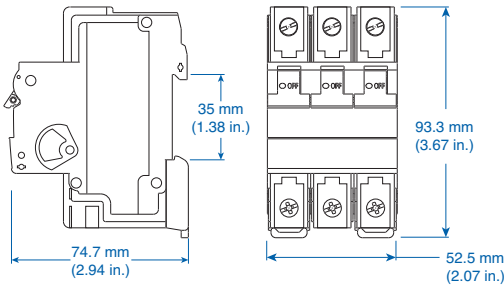
Three Pole
