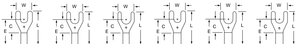
M18-6F M18-8F M18-10F M14-6F M14-8F M14-10F Stud Size 6 8 10 6 8 10 Wire Range 22-18 22-18 22-18 16-14 16-14 16-14
