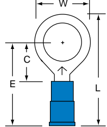
MNG14-38R Stud Size 3/8 Wire Range 16-14
