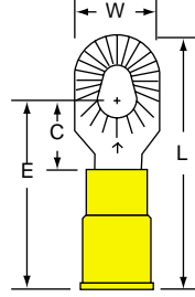
MV10-610R Stud Size 6/8/10 Wire Range 12-10
