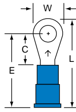
MV14-8R/L Stud Size 8 Wire Range 16-14
