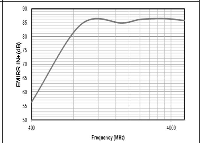
Figure 6. EMIRR IN+ vs. Frequency
