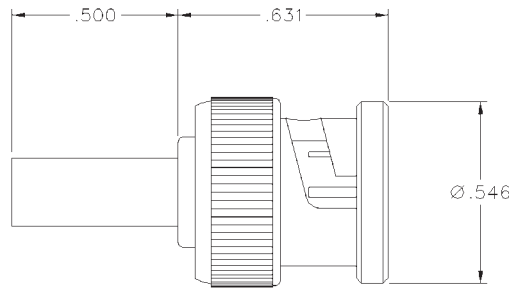
Crimp BNC (M) 3 Piece, solder or crimp captivated contact
