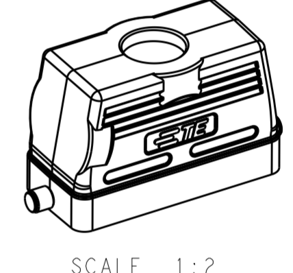
TYPE 2: LOW CONSTRUCTION, TOP ENTRY
