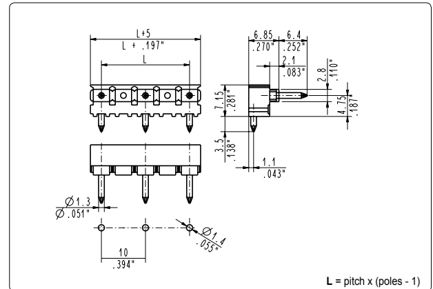
CSM_9A2 90°, side stackable male
