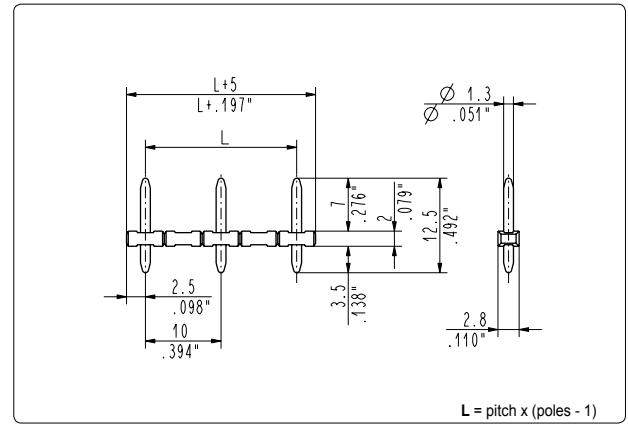
CSM_0A2 straight, side stackable male
