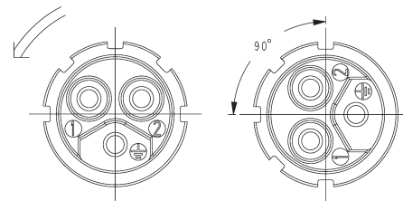
Female / Buchse / Femelle
