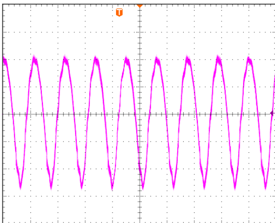
Input Terminal Ripple Current, i_c , at full rated output current and nominal input voltage with 12\mu\text{H} source impedance and 100\mu\text{F} electrolytic capacitor (25 mA/div, 2us/div).
