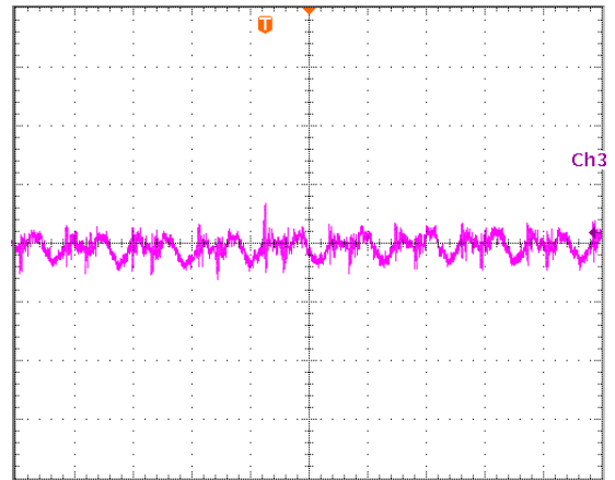
Input reflected ripple current, i_s , through a 12\mu\text{H} source inductor at nominal input voltage and rated load current (5 mA/div, 2us/div)
