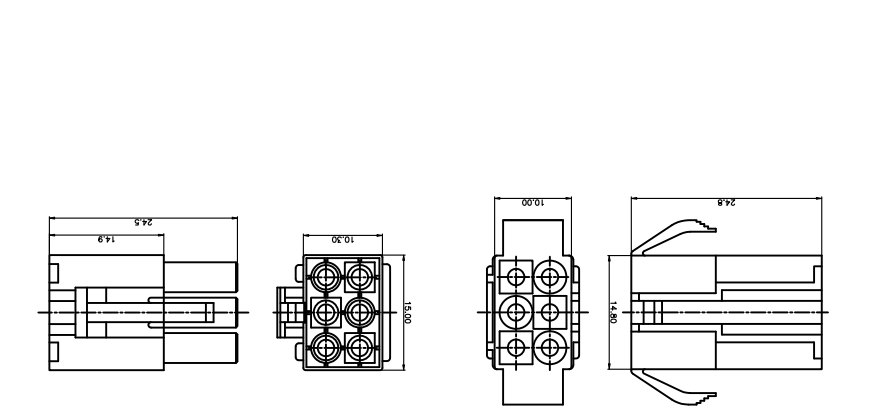
ELR-06P Housing type F MALE (For Female Terminal) FEMALE (For Male Terminal)
