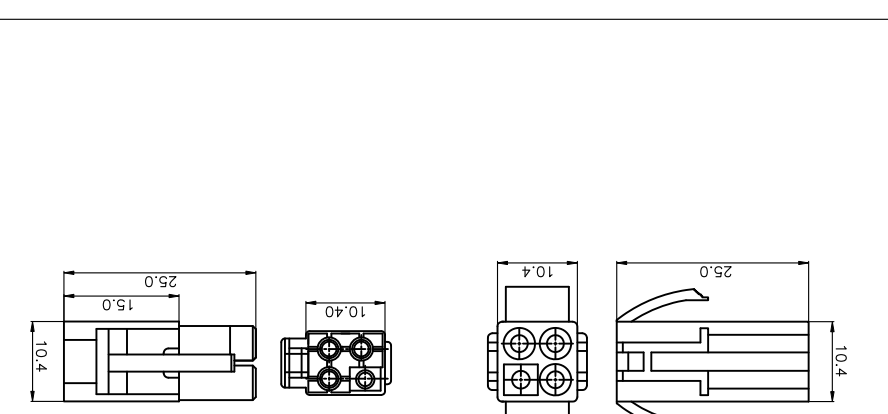
ELR-04P Housing type D MALE (For Female Terminal) FEMALE (For Male Terminal)
