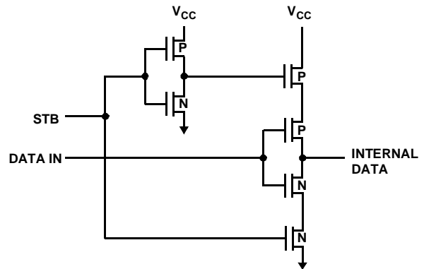
FIGURE 3. 82C82/83H
