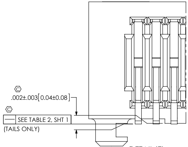
DETAIL 'E' SCALE 8:1
