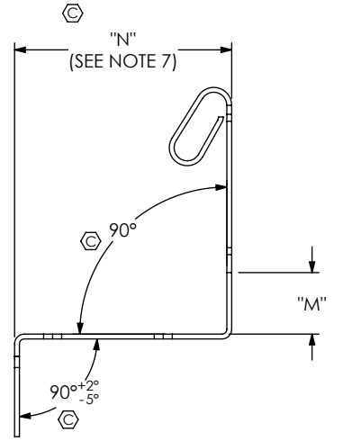
IN-PROCESS 6 (FORM TOP ROW) (C-150-06-X-P SHOWN)
