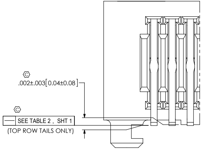
DETAIL 'H' SCALE 8:1
