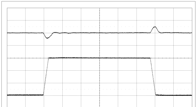
Output voltage response to load current step change (30–90–30 A) at V_i = 12\text{ V} , C_{OUT} = 10 \times 470\ \mu\text{F}/5\ \text{m}\Omega + 10 \times 100\ \mu\text{F} , di/dt = 2\ \text{A}/\mu\text{s} , ASCR Gain = 300 and ASCR Residual = 90. Scale from top: 50 mV/div, 20 A/div, 100 \mu\text{s} /div. Note: Sense pins are connected to load.
