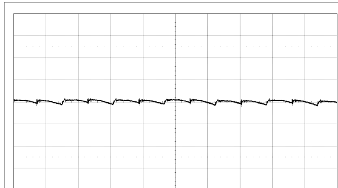
Fundamental output voltage ripple at V_i = 12\text{ V} , I_o = \text{max } I_o , C_{OUT} = 10 \times 470\ \mu\text{F}/5\ \text{m}\Omega + 10 \times 100\ \mu\text{F} . Scale: 10 mV/div, 2 \mu\text{s} /div, 20 MHz bandwidth. See section Output Ripple and Noise.
