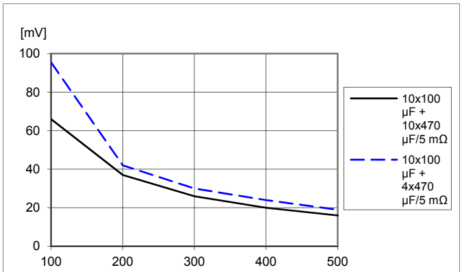
Load transient peak voltage deviation vs. ASCR gain and external capacitance. Step (30–90–30 A). V_I = 12\text{ V} , V_O = 1.0\text{ V} , f_{sw} = 320\text{ kHz} , ASCR residual =90, di/dt = 2\text{ A}/\mu\text{s} . ASCR gain changed by PMBus command ASCR_CONFIG.
