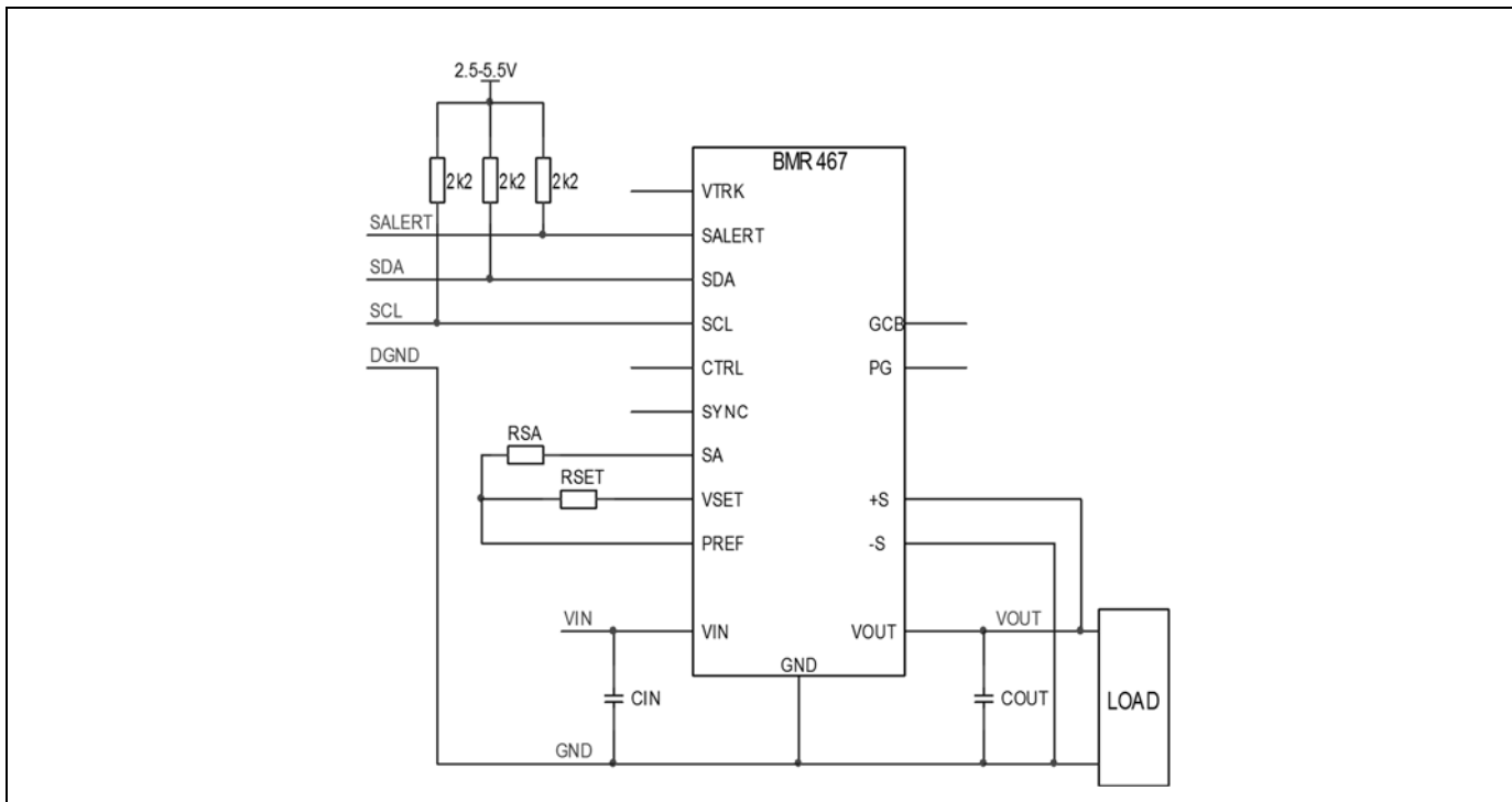
Standalone operation with PMBus communication.
