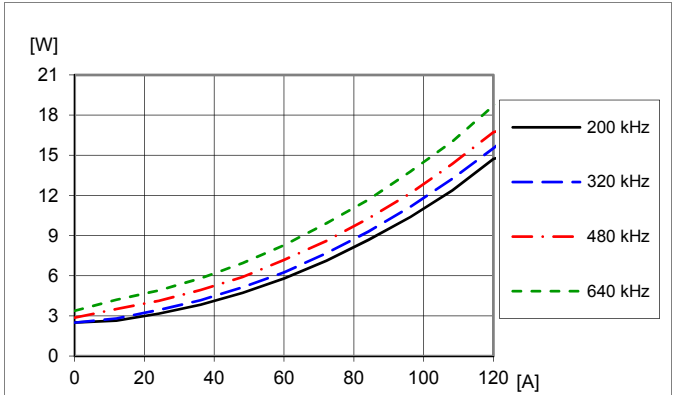
Dissipated power vs. load current and switching frequency at V_I = 12\text{ V} , V_O = 1.0\text{ V} , C_O = 10 \times 470\text{ }\mu\text{F}/5\text{ m}\Omega + 10 \times 100\text{ }\mu\text{F} . Frequency changed by PMBus command FREQUENCY_SWITCH.
