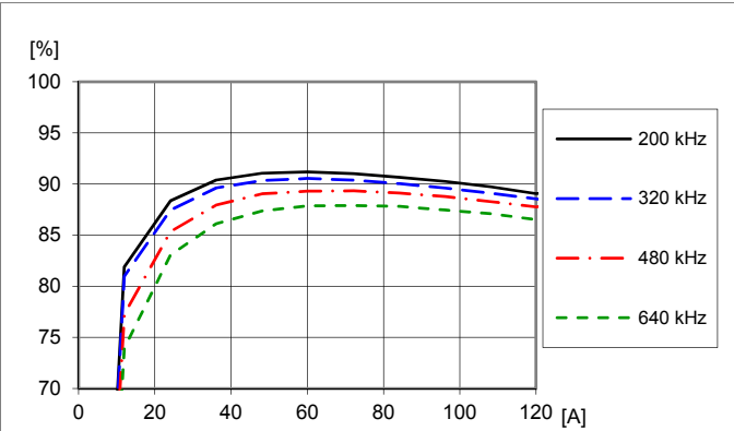
Efficiency vs. load current and switching frequency at V_I = 12\text{ V} , V_O = 1.0\text{ V} , C_O = 10 \times 470\text{ }\mu\text{F}/5\text{ m}\Omega + 10 \times 100\text{ }\mu\text{F} . Frequency changed by PMBus command FREQUENCY_SWITCH.
