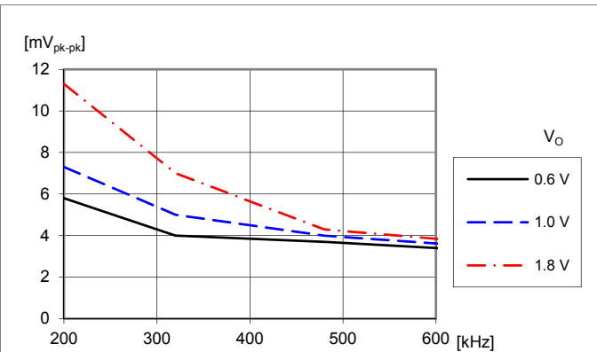
Output voltage ripple V_{pk-pk} vs. switching frequency at V_I = 12\text{ V} , I_O = \text{max } I_O , C_O = 10 \times 470\text{ }\mu\text{F}/5\text{ m}\Omega + 10 \times 100\text{ }\mu\text{F} . Frequency changed by PMBus command FREQUENCY_SWITCH.
