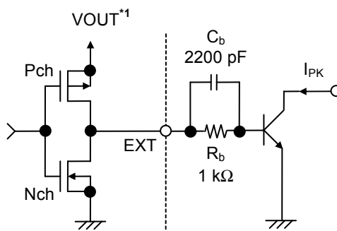
Figure 18 External Transistor Peripheral Circuit
