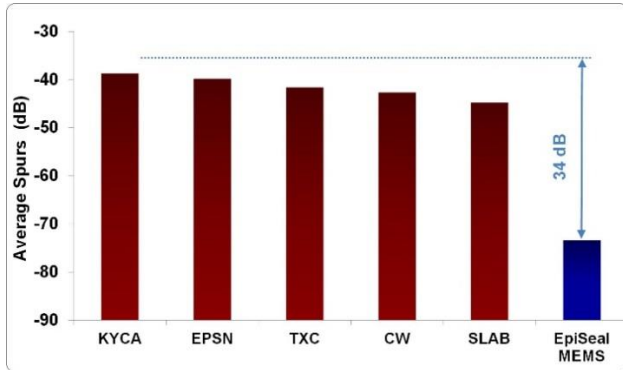
Figure 5. Vibration Robustness [5]
