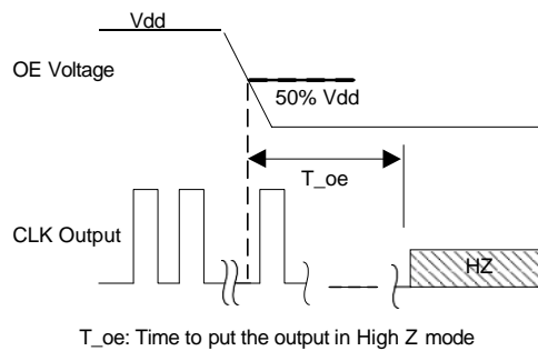
Figure 7. OE Disable Timing (OE Mode Only)
