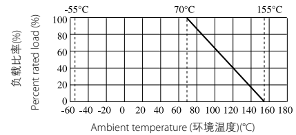
Derating Curve (降功率曲线)
