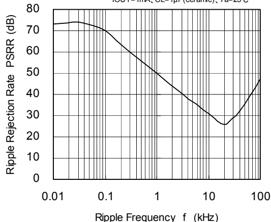
XC6202P332 (3.3V)
