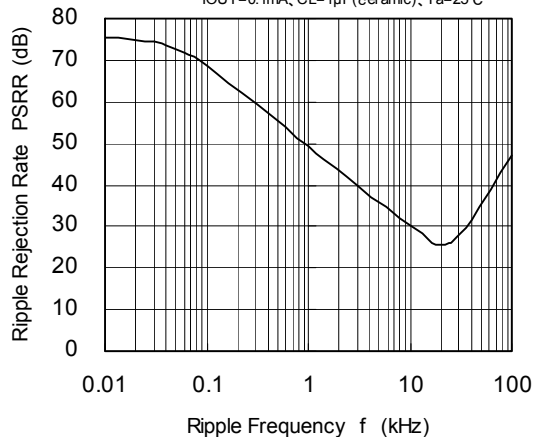
XC6202P332 (3.3V)
