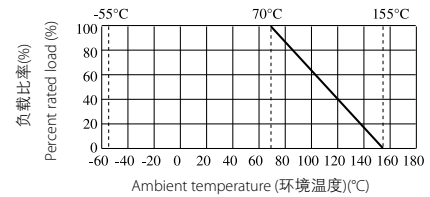
Derating Curve (降功率曲线)
