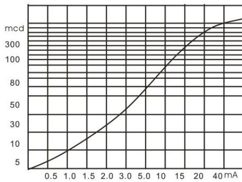
Input mA/mcd curve
