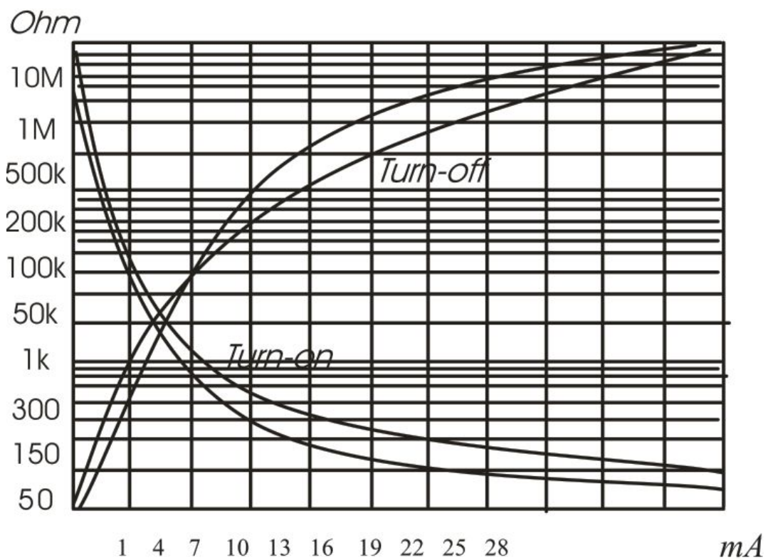
Input mA/ohm curve
