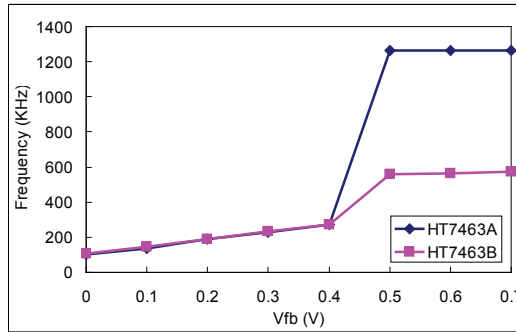
f sw vs. V FB (HT7463A and HT7463B)
