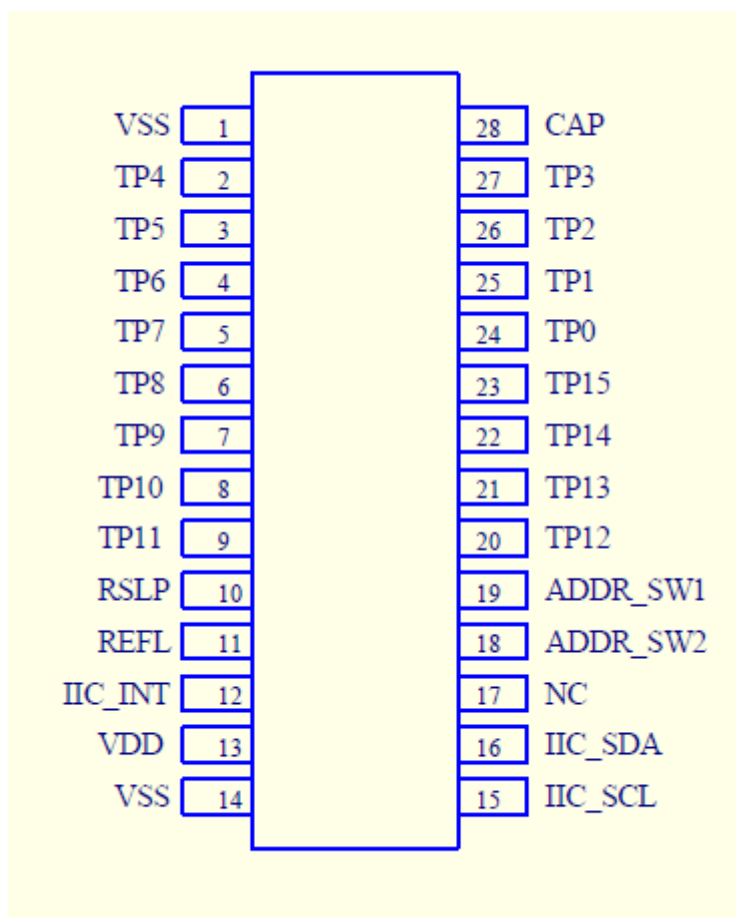
Figure5. pin define for IC package
