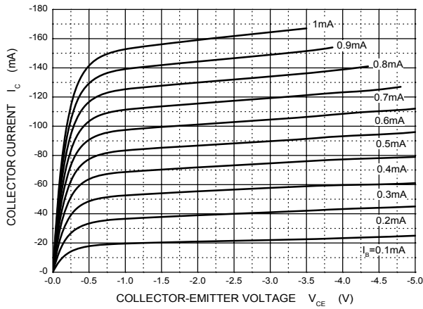
Static Characteristic
