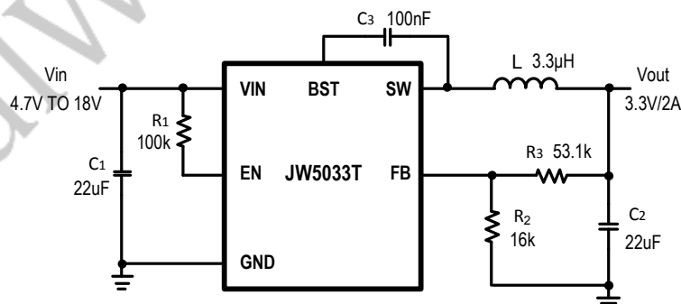
3.3V/2A Step Down Regulator
