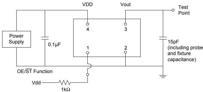
Figure 2. Test Circuit
