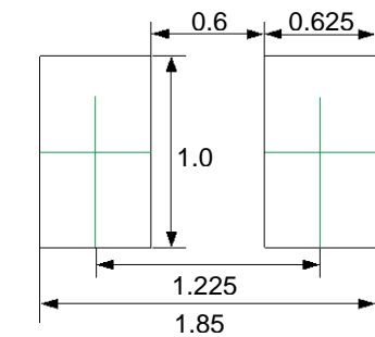
Recommended Soldering Pad
