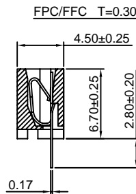
FPC/FFC T=0.30
