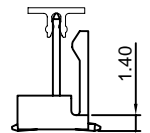
TYPICAL END VIEW FOR 2P THRU 7P
