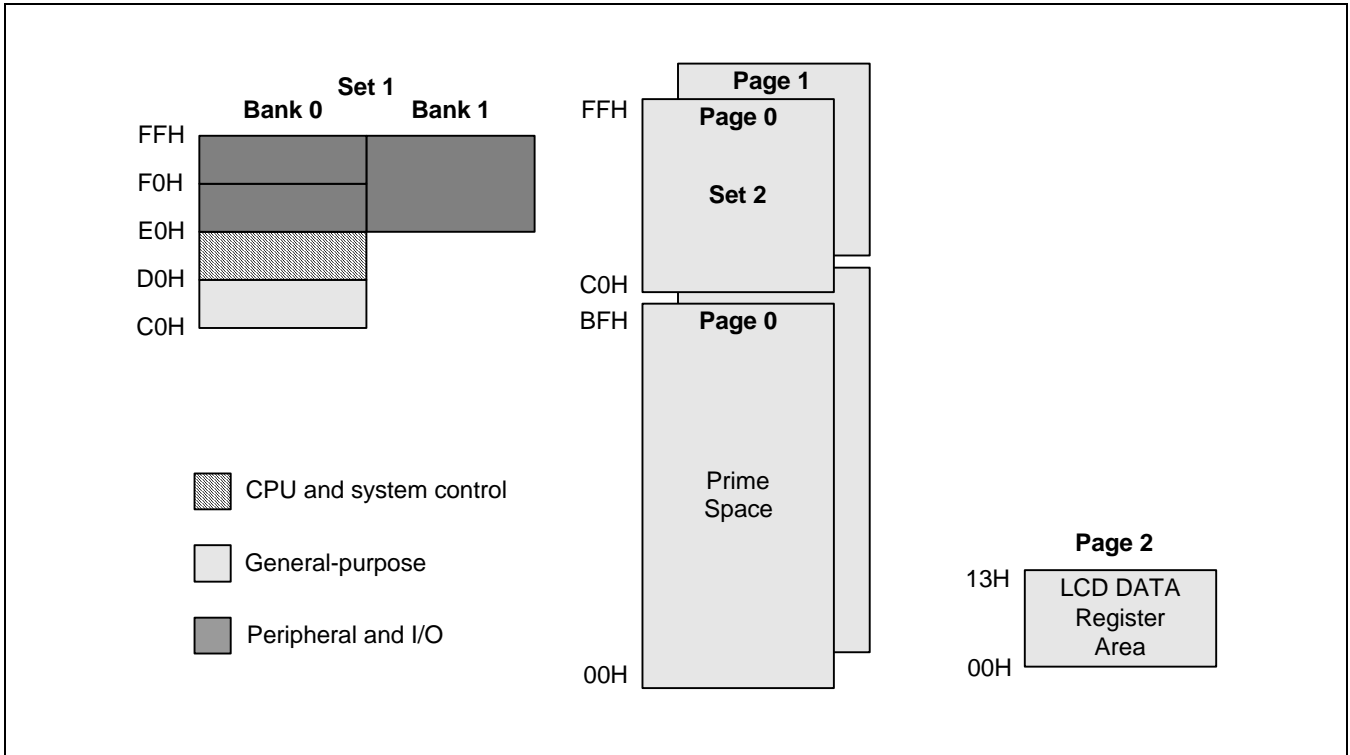
Figure 2-6. Set 1, Set 2, Prime Area Register(S3C8419X/F8419X)
