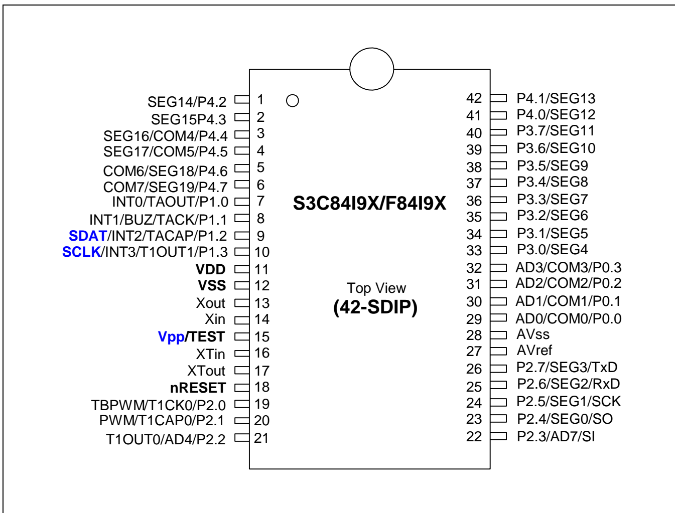
Figure 1-3. S3C8419X/F8419X Pin Assignment (42-pin SDIP)
