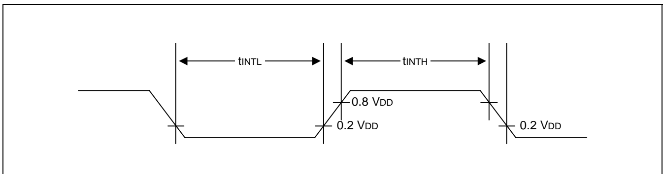
Figure 21-1. Input Timing for External Interrupts (Ports 2)
