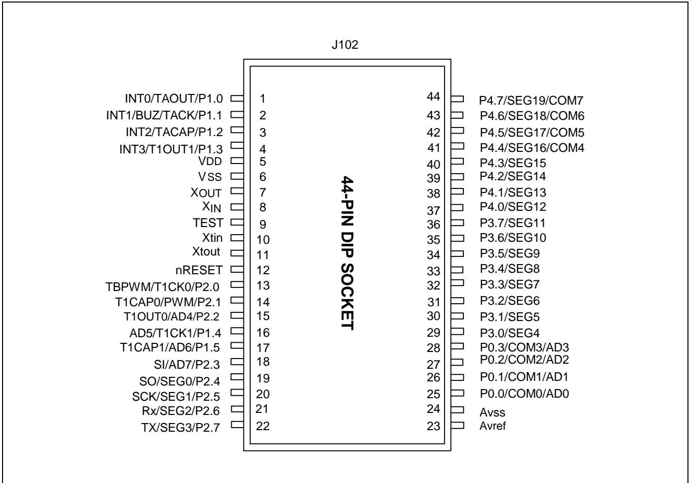
Figure 23-4. 44-Pin Connector Pin Assignment for TB8419
