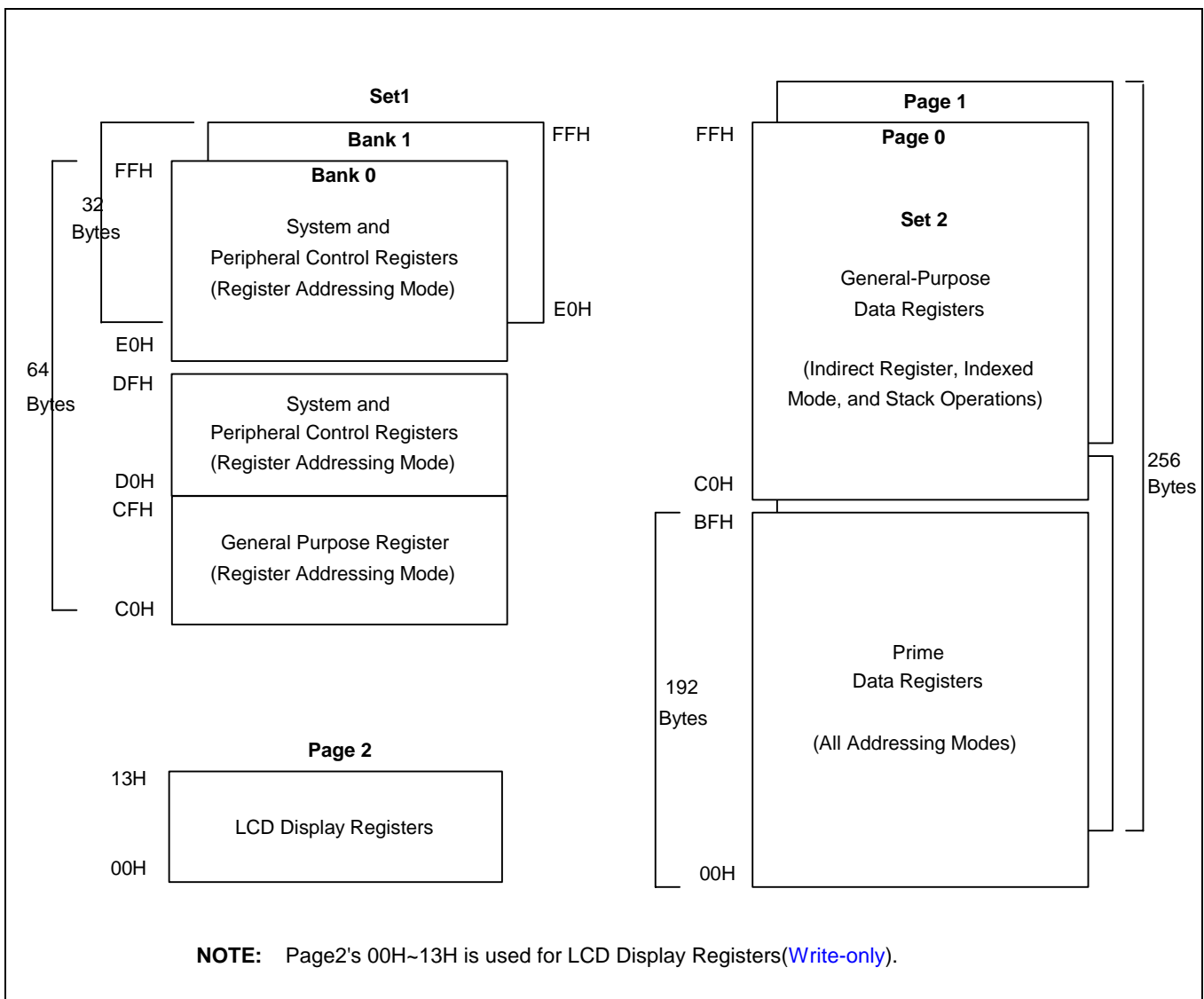
Figure 2-3. Internal Register File Organization of S3F8419X/C8419X
