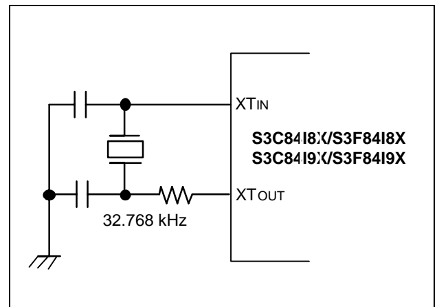
Figure 7-2. Sub-System Oscillator Circuit (Crystal Oscillator)
