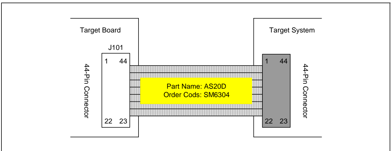
Figure 23-6. TB8419 Adapter Cable for 44pin Connector Package
