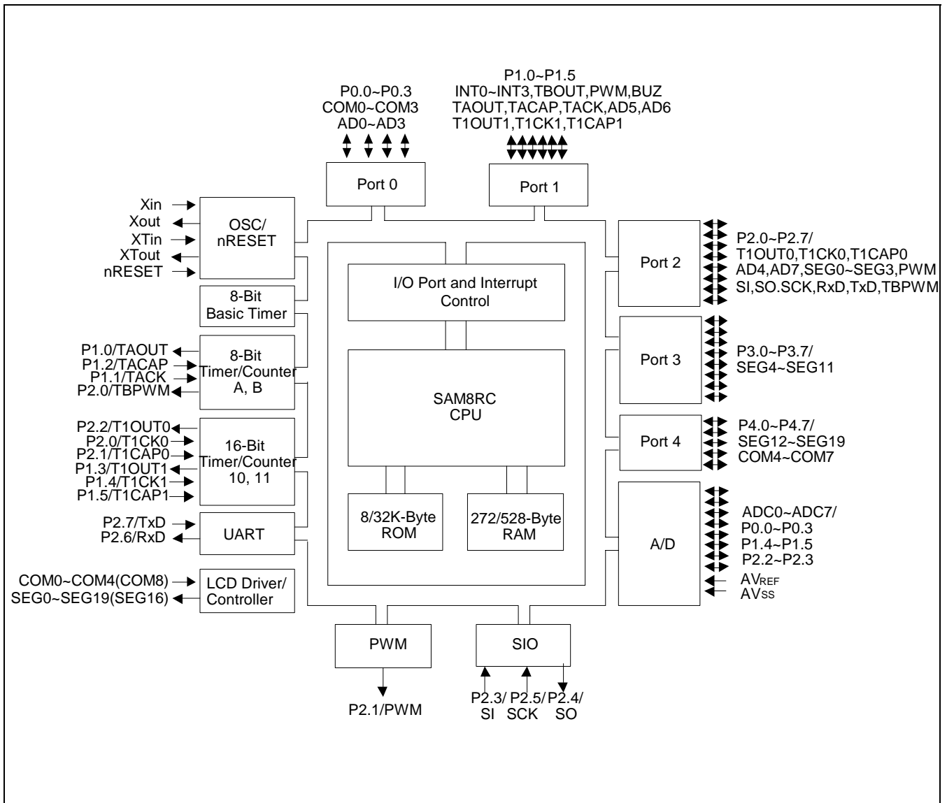
Figure 1-1. S3C8418/F8418/C8419/F8419 Block Diagram
