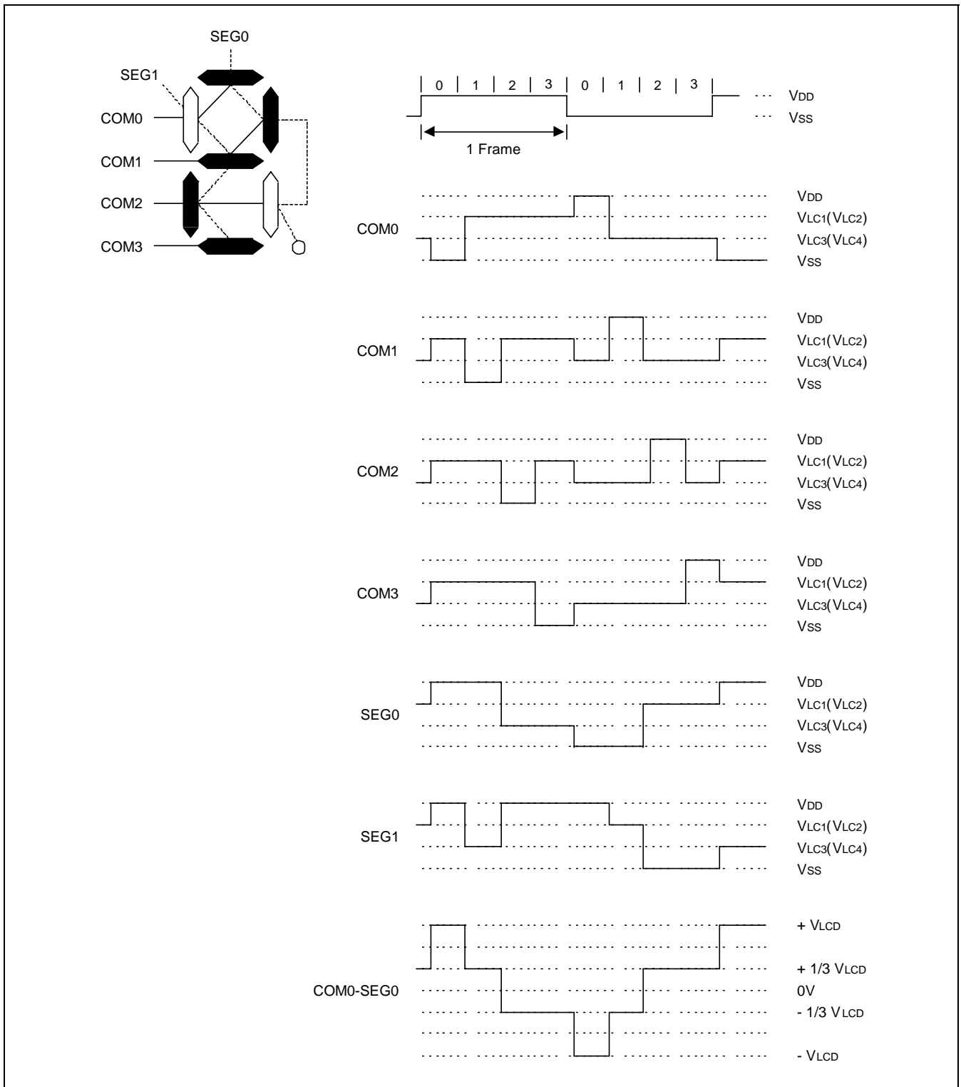
Figure 18-8. LCD Signal Waveforms (1/4 Duty, 1/3 Bias)
