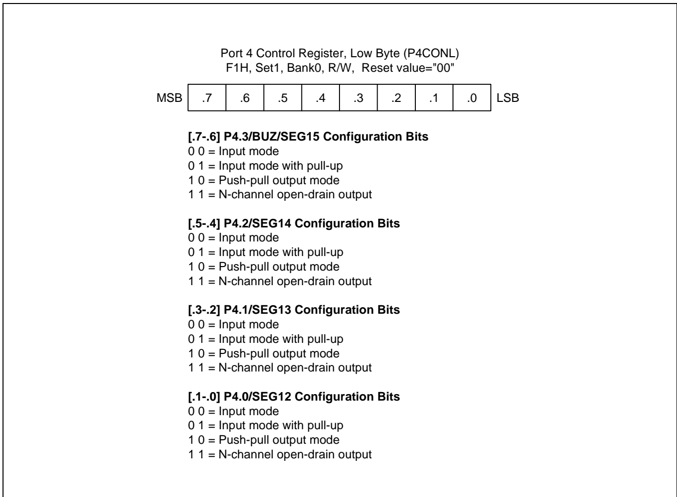
Figure 9-12. Port 4 Low-Byte Control Register (P4CONL)
