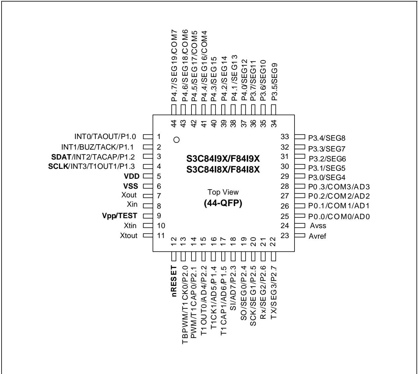
Figure 1-2. S3C8418X/F8418X/C8419X/F8419X Pin Assignment (44-pin QFP)
