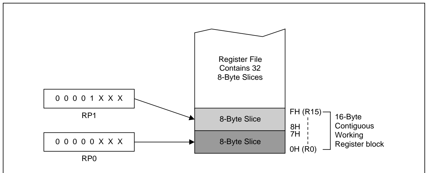
Figure 2-9. Contiguous 16-Byte Working Register Block
