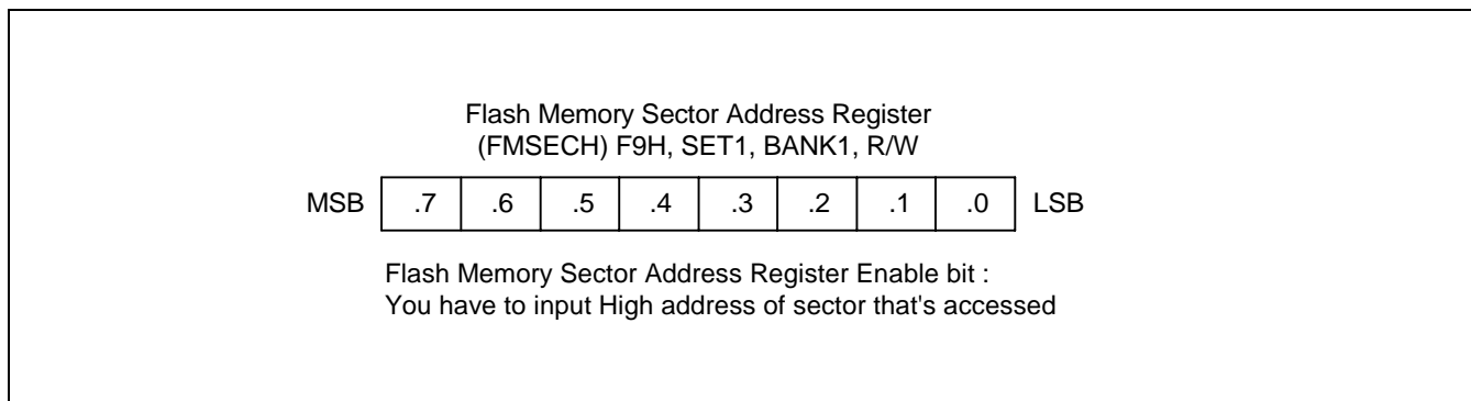
Figure 20-4. Flash Memory Sector Address Register (FMSECH)
