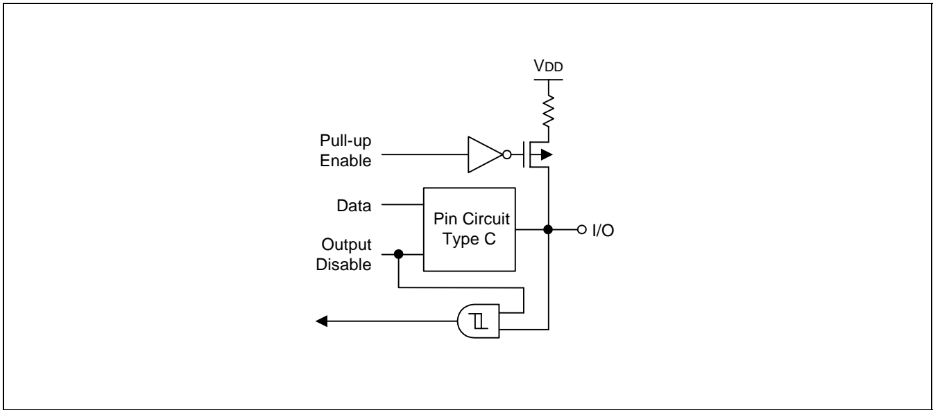
Figure 1-6. Pin Circuit Type D
