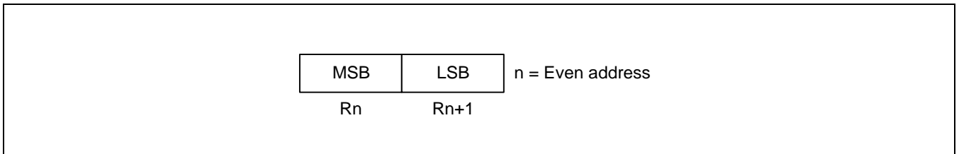
Figure 2-11. 16-Bit Register Pair
