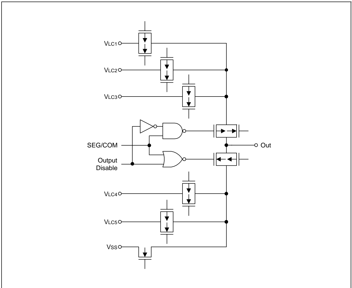
Figure 1-9. Pin Circuit Type H-4
