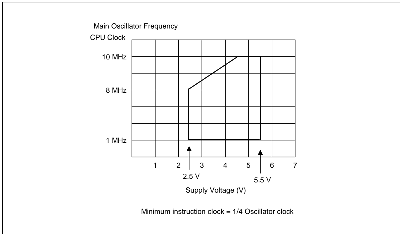
Figure 21-8. Operating Voltage Range
