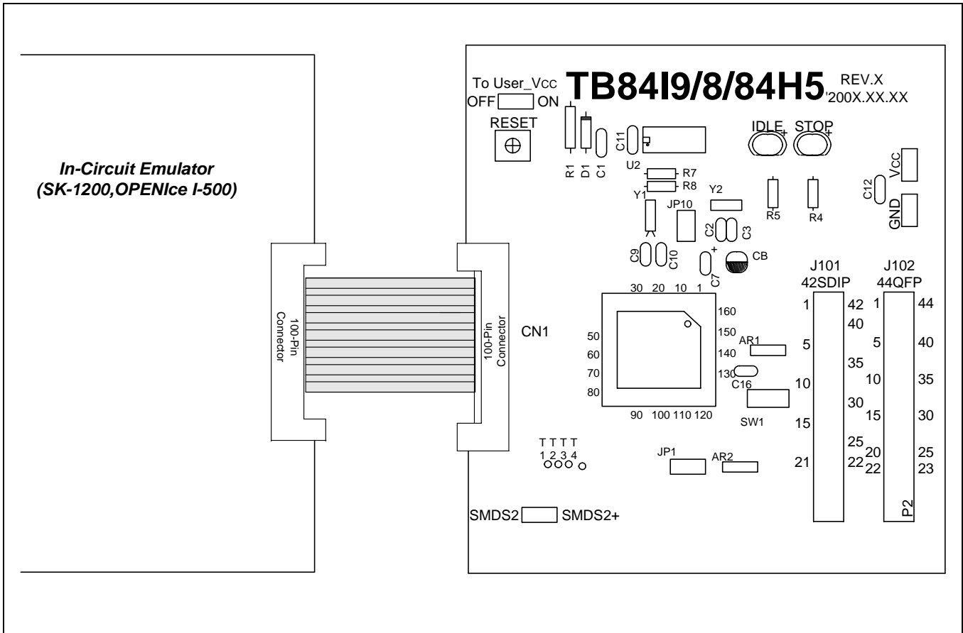
Figure 23-2. S3F8419X/S3F8418X Target Board Configuration
