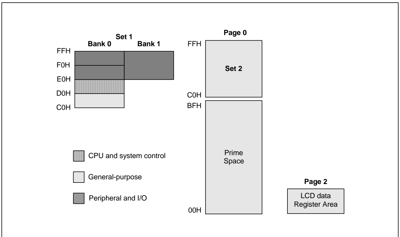
Figure 2-7. Set 1, Set 2, Prime Area Register (S3C8418X/F8418X)
