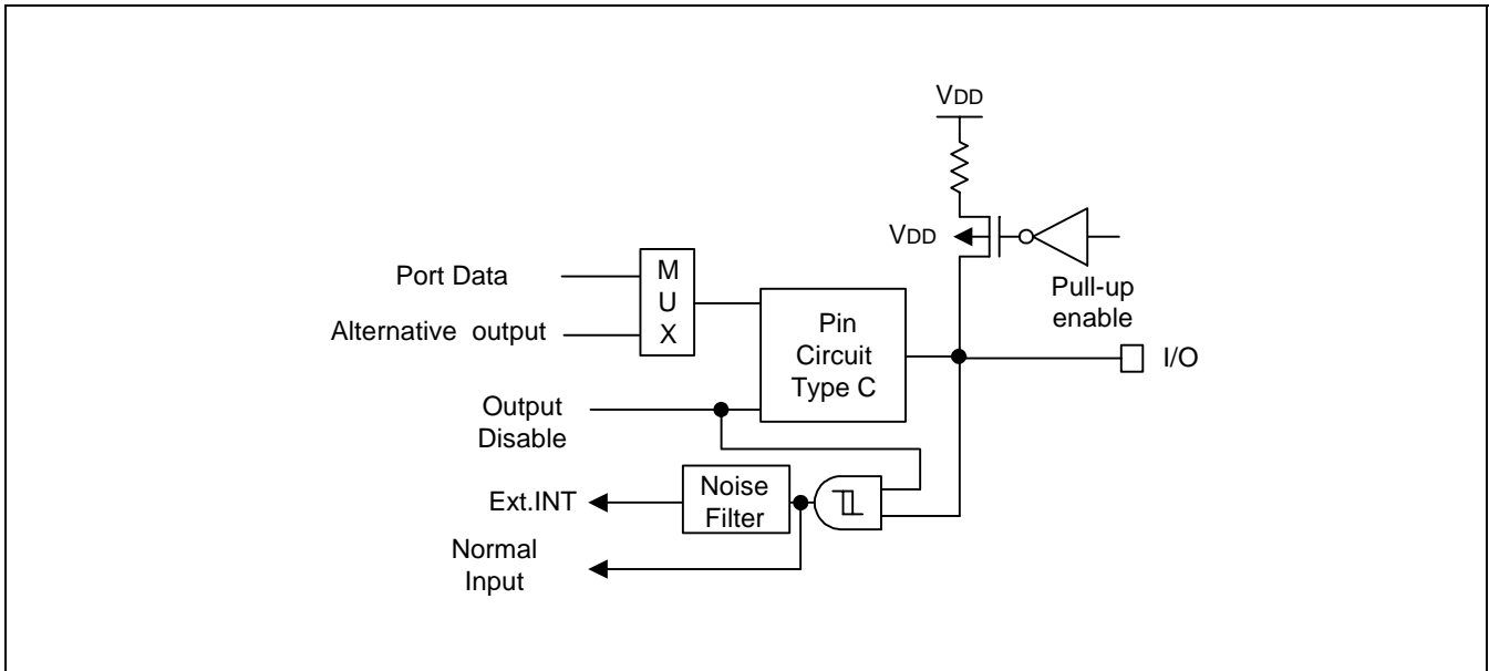
Figure 1-7. Pin Circuit Type D-5 (P1.0-P1.3)
