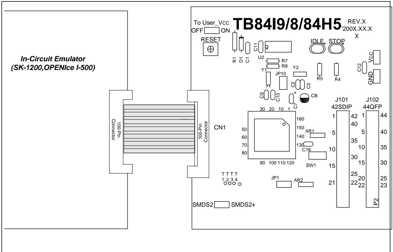
Figure 23-2. S3F8419X/S3F8418X Target Board Configuration
