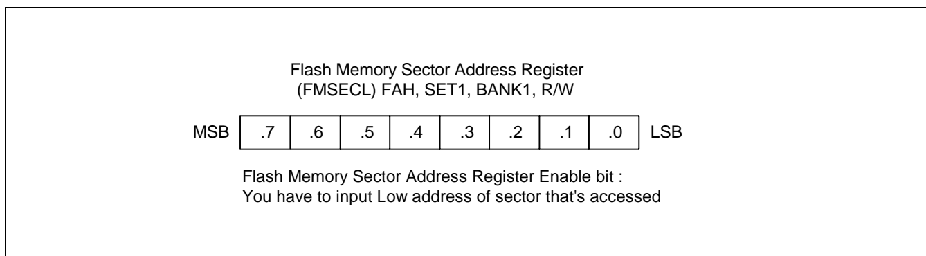
Figure 20-5. Flash Memory Sector Address Register (FMSECL)
