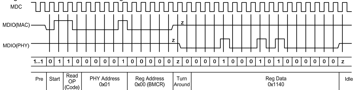
Figure 6. Read Cycle
