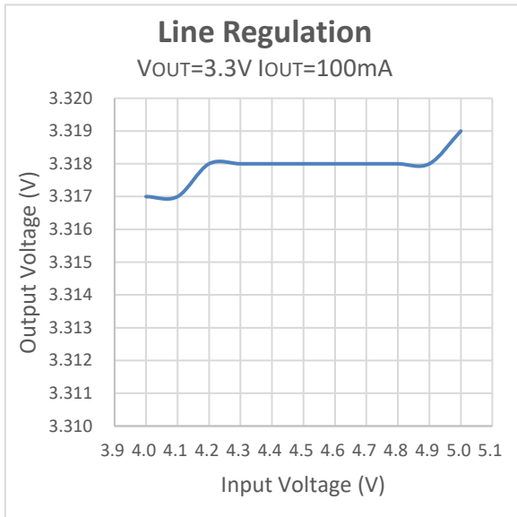
Line Regulation V OUT =3.3V
