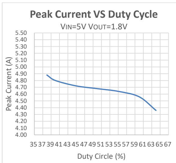
Peak Current VS Duty Circle
