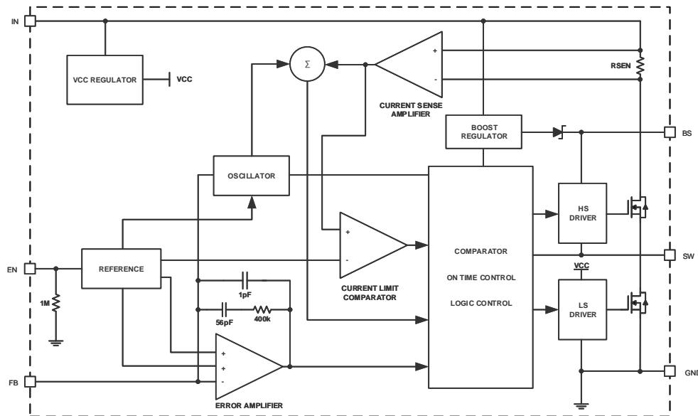
Figure 2. RY8120 Block Diagram
