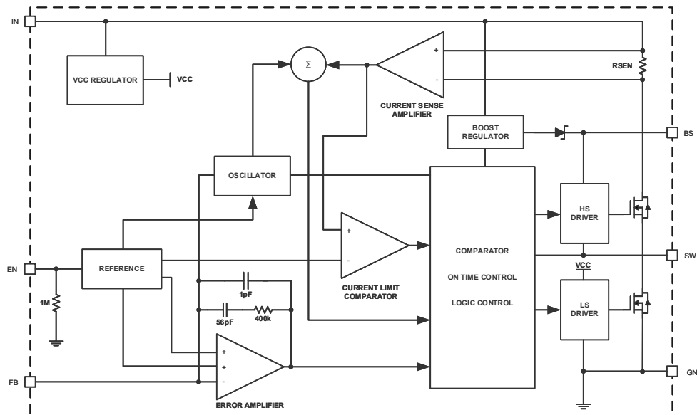
Figure 2. RY3825 Block Diagram
