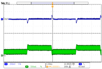
Load Transient
