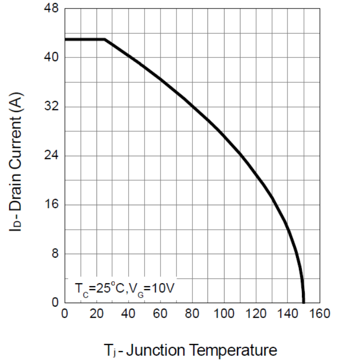
Drain Current
