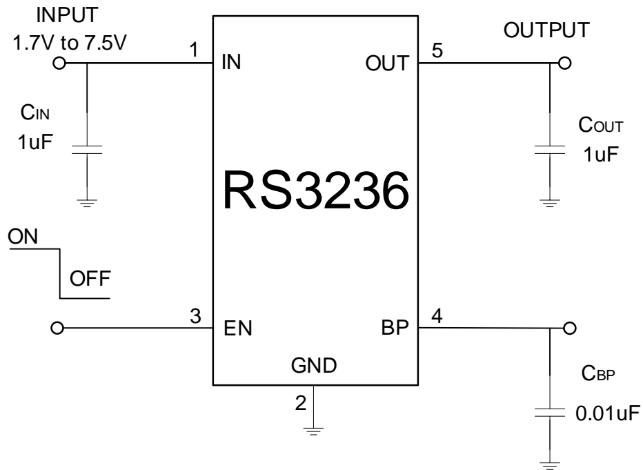
Typical Circuit
