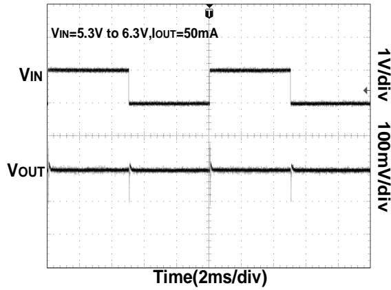
Line-Transient Response
