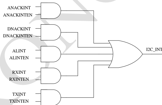
Figure 123 I2C 中断
