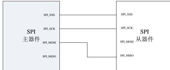
Figure 127 3 线单从机互连
