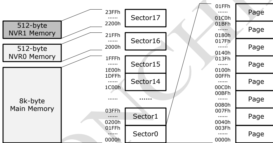
Figure 13 FLASH Memory
