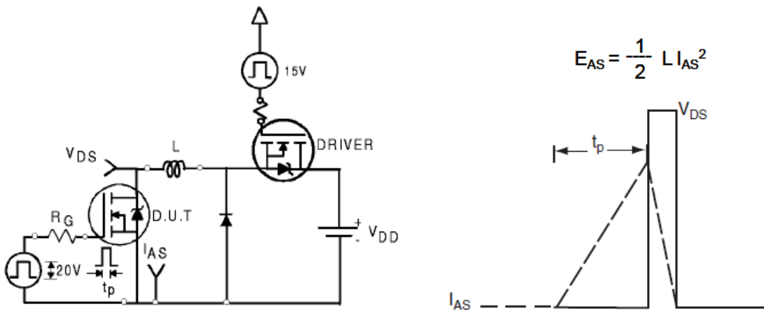
Fig. 21. Unclamped Inductive switching test circuit & waveform
