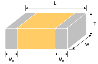
Fig. 5.1 The outline of MLCC
