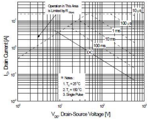
Figure 9-2. Maximum Safe Operating Area for TSP5N65M
