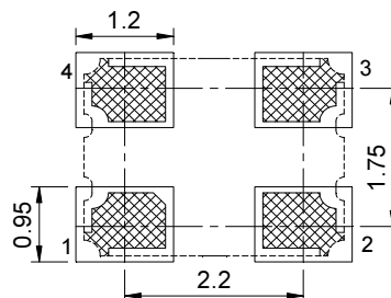
Land Pattern Layout
