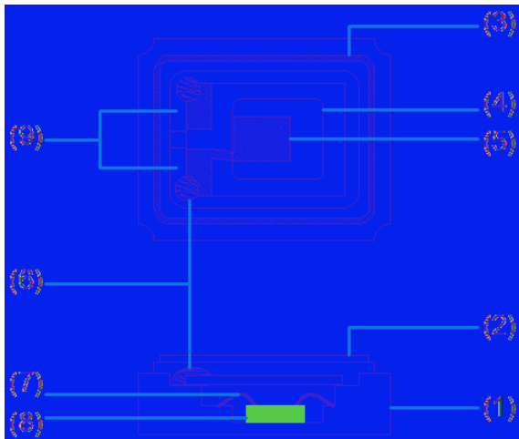
Reference drawing
