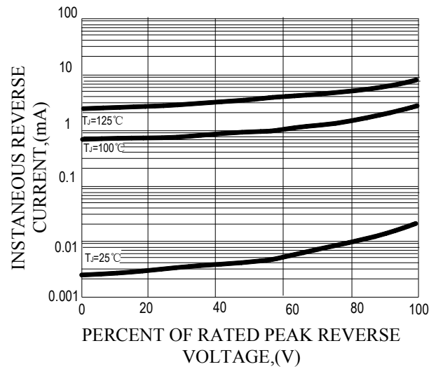
FIG.4-TYPICAL REVERSE CHARACTERISTICS
