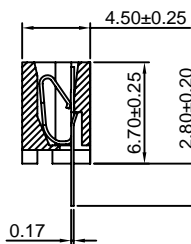
FPC/FFC T=0.30
