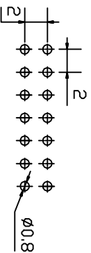
PCB LAYOUT
