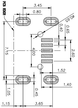
RECOMMENDED PCB LAYOUT (TOL: ±0.05)
