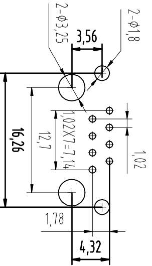
PC Board Layout Component Side Shown
