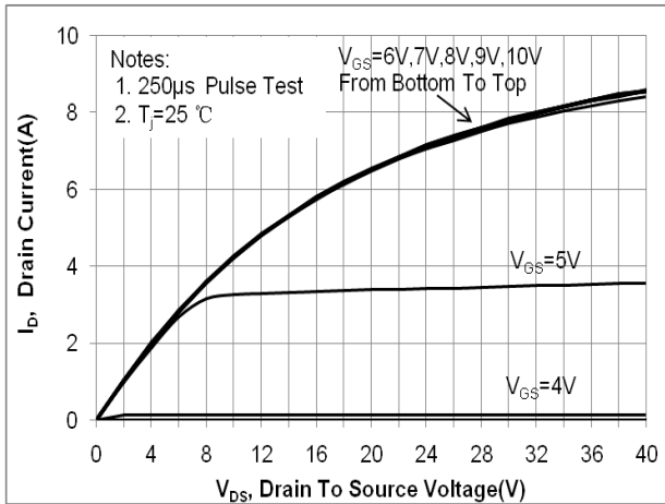
Fig. 1. On-state characteristics
